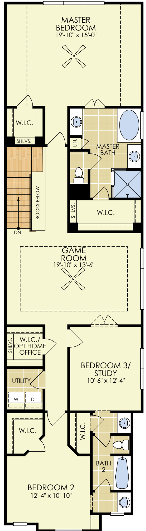
SECOND FLOOR
