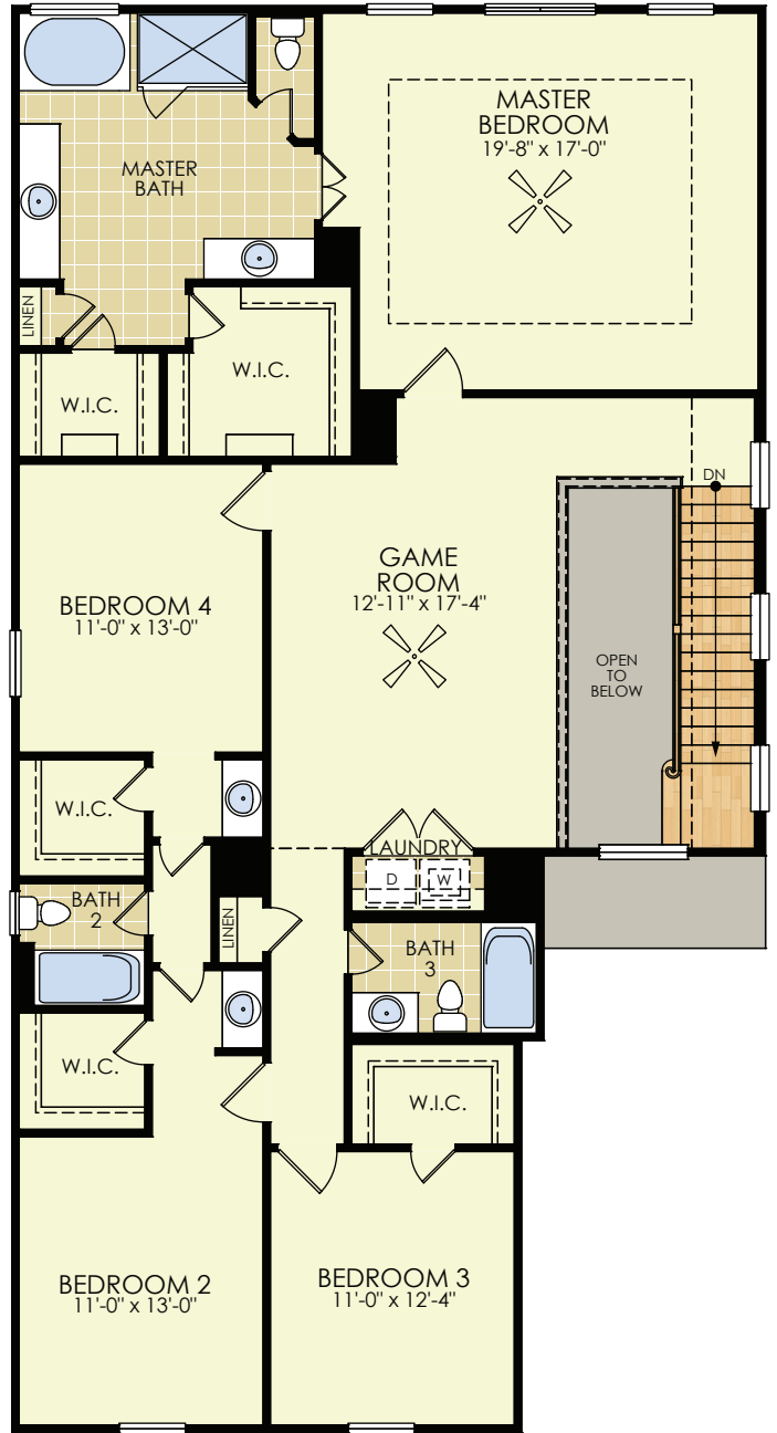
SECOND FLOOR
