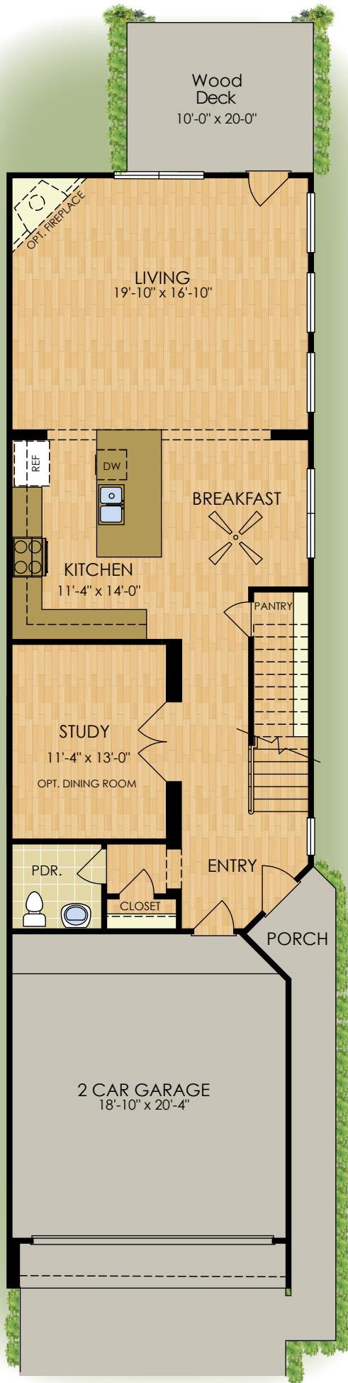
FIRST FLOOR
